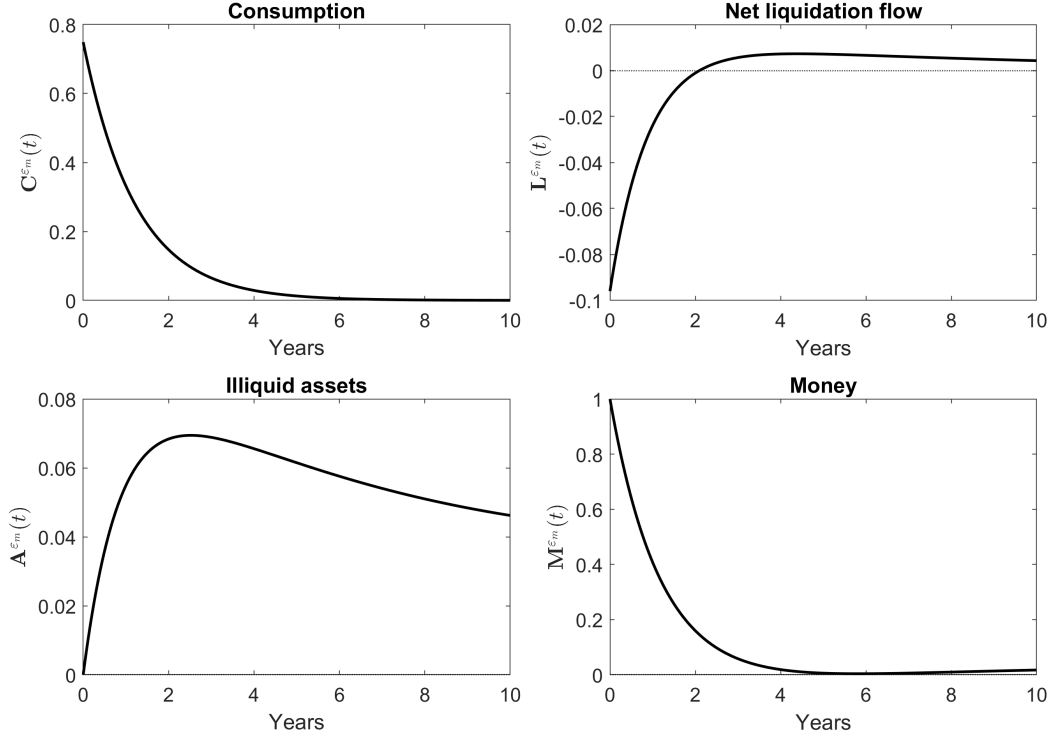
Figure 6: The Functional Sufficient Statistic
