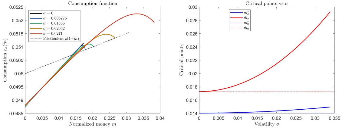
Figure 5: Consumption Function and Critical Points Under Income Risk
